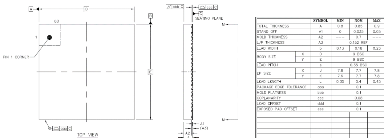
Figure 2-1 SG2002 package dimensions, top view
